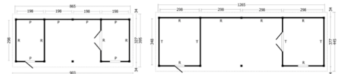
ZADELDAK HAMAR, TYPE 12 ■ 903x395cm / 1303x445cm
