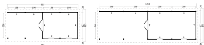
ZADELDAK HAMAR, TYPE 11 ■ 903x395cm / 1303x445cm
