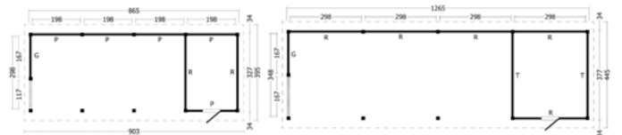
ZADELDAK HAMAR, TYPE 10 ■ 903x395cm / 1303x445cm
