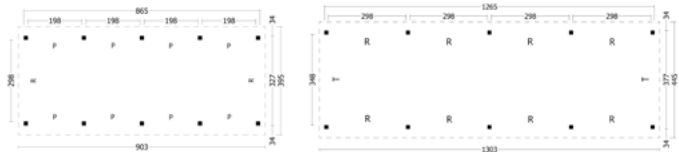
ZADELDAK HAMAR, TYPE 9 ■ 903x395cm / 1303x445cm
